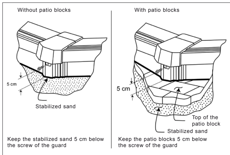
FIG.3 - WITH/WITOUT PATIO BLOCKS
