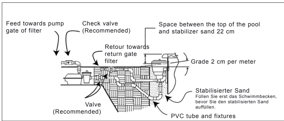
FIG. 2 SPECIFIC INSTALLATION
